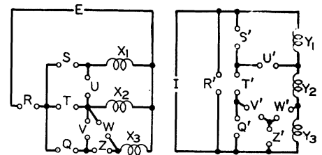
Figure 21 (left). Simple constant-voltage system
